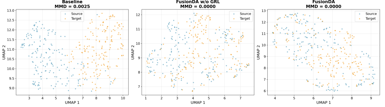
Figure 3.5: UMAP visualization of the backbone feature space on 175 clear and 175 foggy samples. Left: the Baseline shows a clear separation between the two domains along the UMAP-1 axis. Middle: FusionDA w/o GRL - the two distributions are substantially mixed and MMD drops to approximately 0. Right: FusionDA (full) - the two distributions become more uniformly arranged in terms of local structure, even though the MMD is already saturated.
