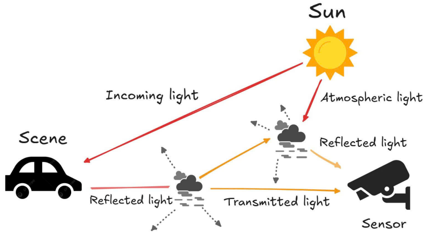
Figure 1: The atmospheric scattering model. Light from the source illuminates the scene; part of it is reflected, while another part is scattered by fog particles and absorbed before reaching the sensor. In addition, ambient light produced by multiple scattering reaches the sensor directly, brightening the captured image and reducing its contrast.
